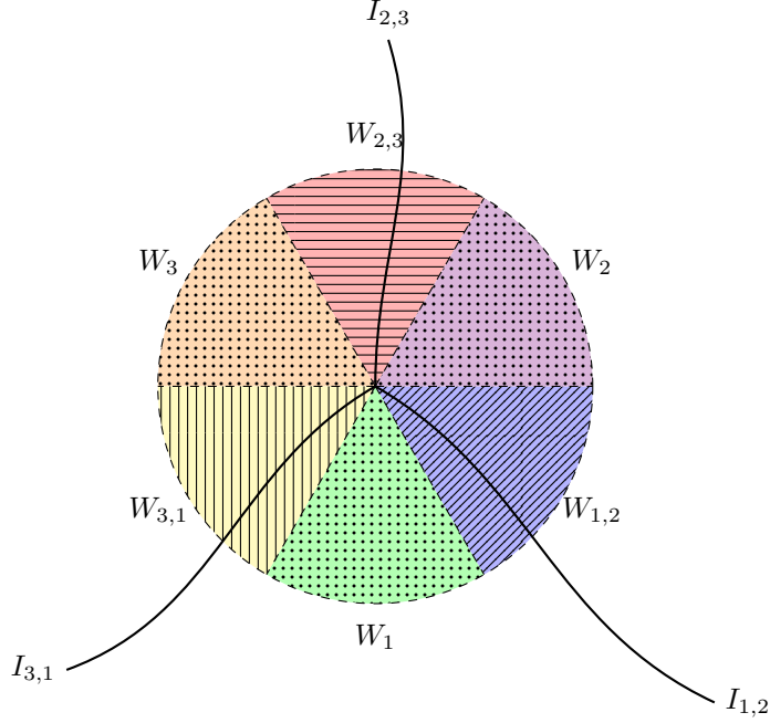
FIGURE 3. A cross-section orthogonal to the triple line illustrating the wedge decomposition in Definition 16. The “interpolation wedges” are marked with a dotted pattern, the “interface wedges” with striped patterns.
